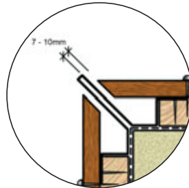
DETAIL 5.
