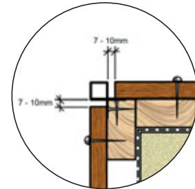
DETAIL 6.
