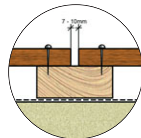
DETAIL 11.
