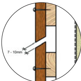
DETAIL 12.
